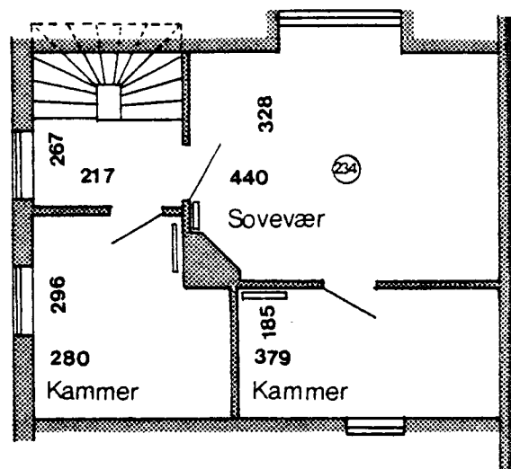
1 Sals plan
