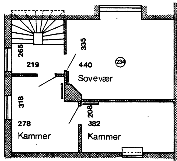
1 Sals plan
