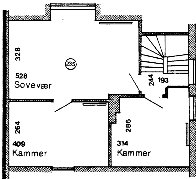
1 Sals plan
