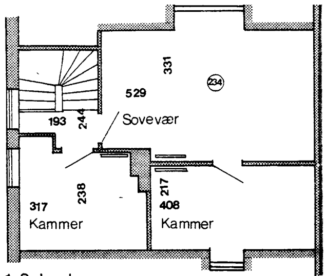
1 Sals plan
