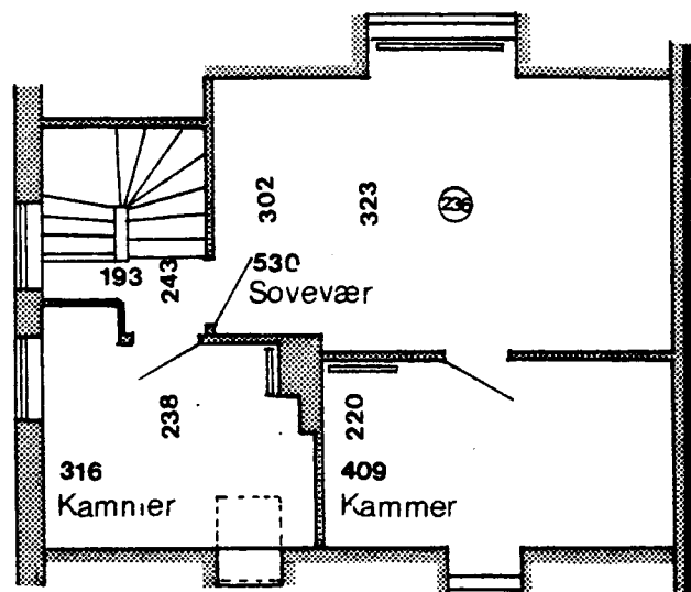
1 Sals plan
