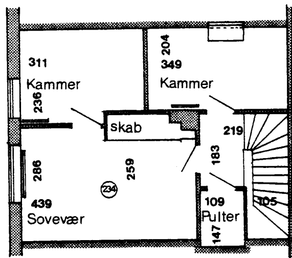
1 Sals plan
