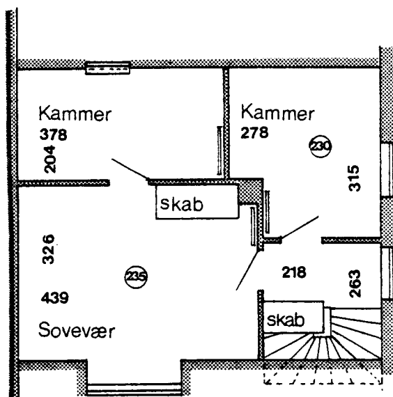
1 Sals plan
