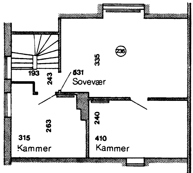
1 Sals plan
