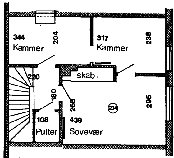
1 Sals plan
