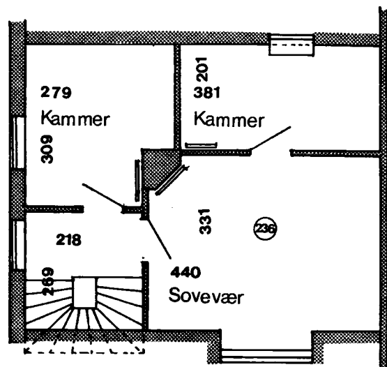
1' Sals plan
