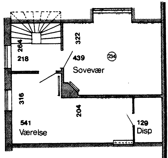
1 Sals plan
