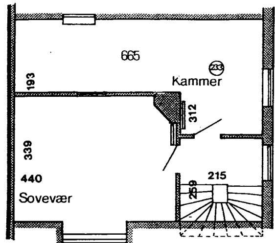
1 Sals plan
