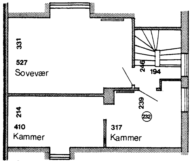
1 Sals plan
