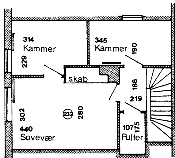
1 Sals plan
