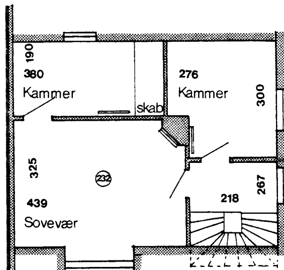
1 Sals plan
