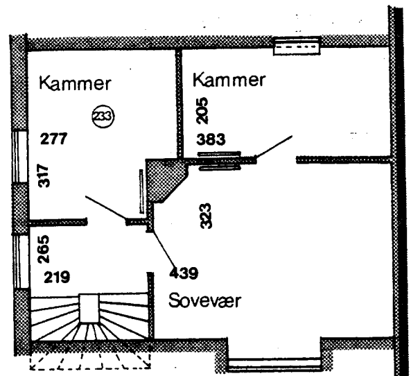
1 Sals plan
