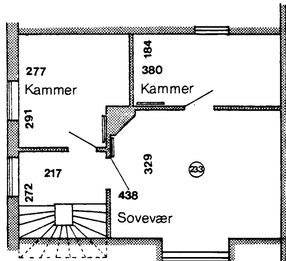
1 Sals plan
