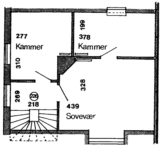
1 Sals plan
