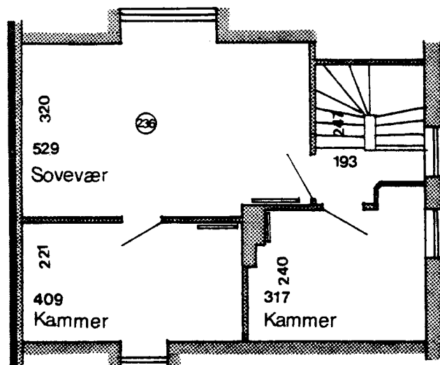
1 Sals plan
