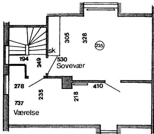
1 Sals plan
