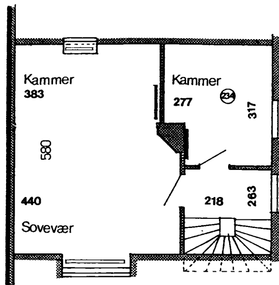
1 Sals plan
