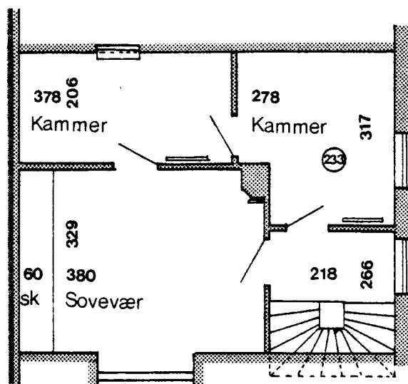
1 Sals plan
