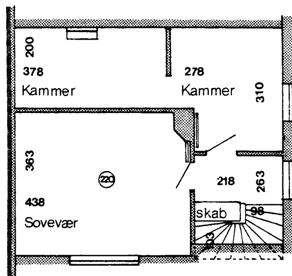
1 Sals plan
