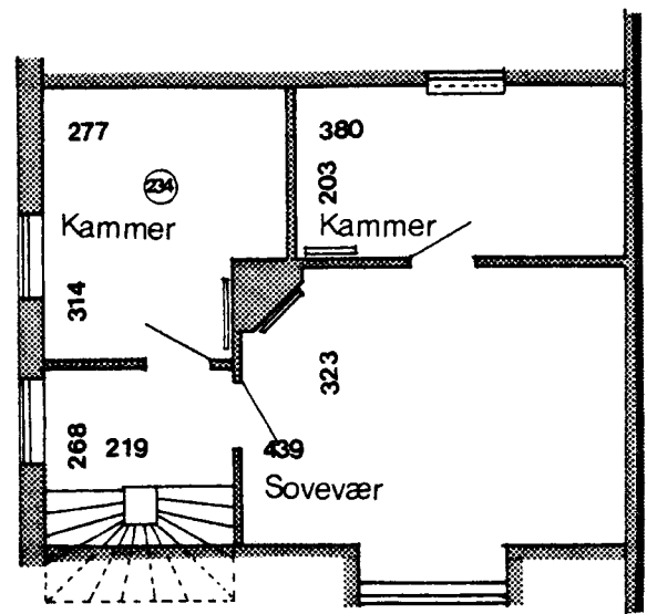
1 Sals plan
