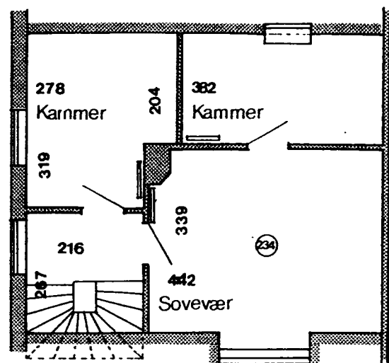
1 Sals plan
