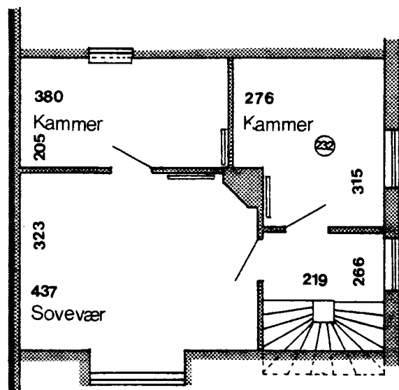
1 Sals plan
