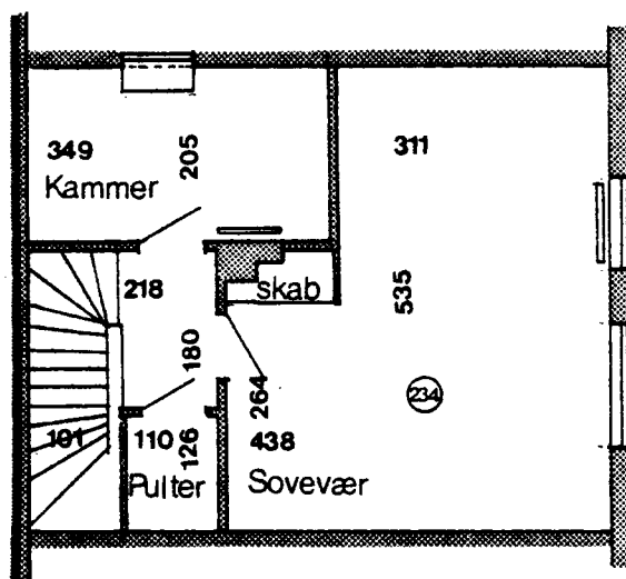
1 Sals plan
