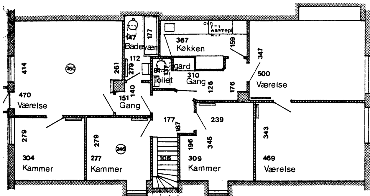
1. Sals plan
