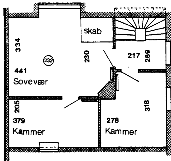
1 Sals plan
