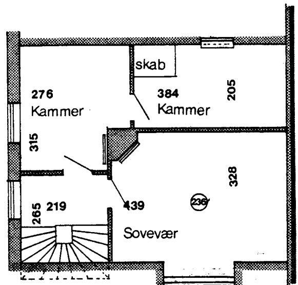
1 Sals plan
