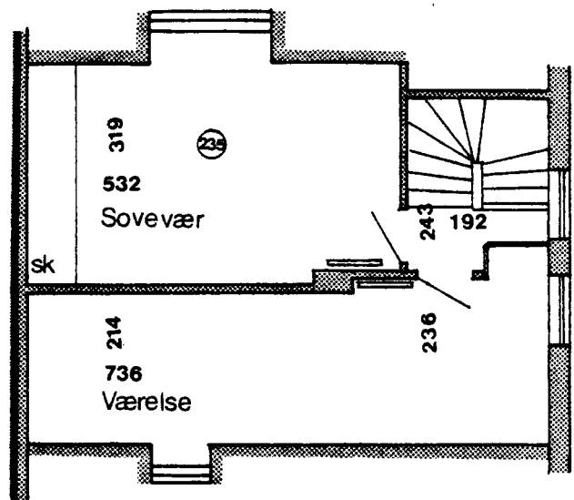
1 Sals plan
