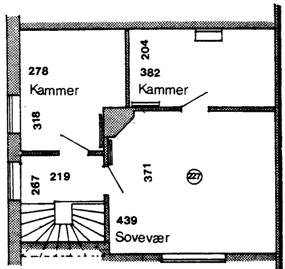
1 Sals plan
