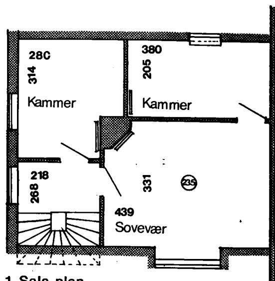
1 Sals plan
