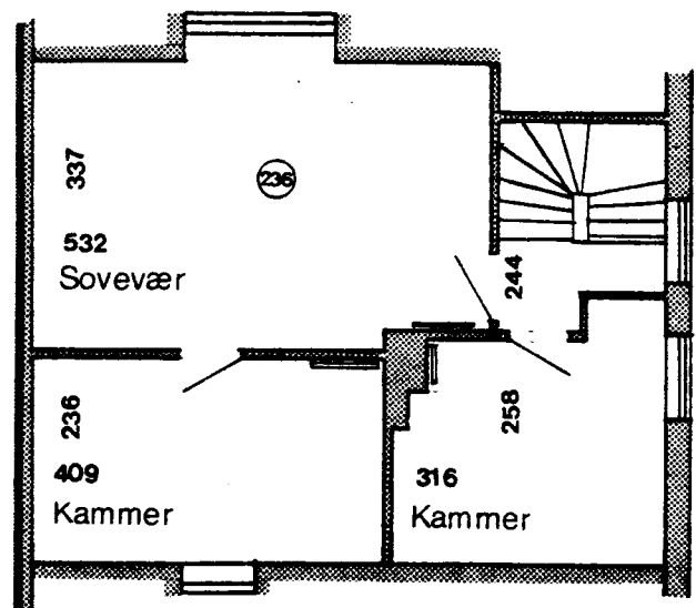
1 Sals plan
