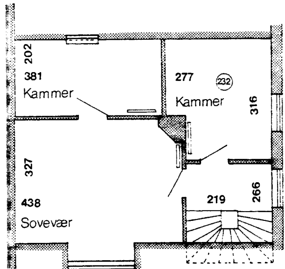
1 Sals plan
