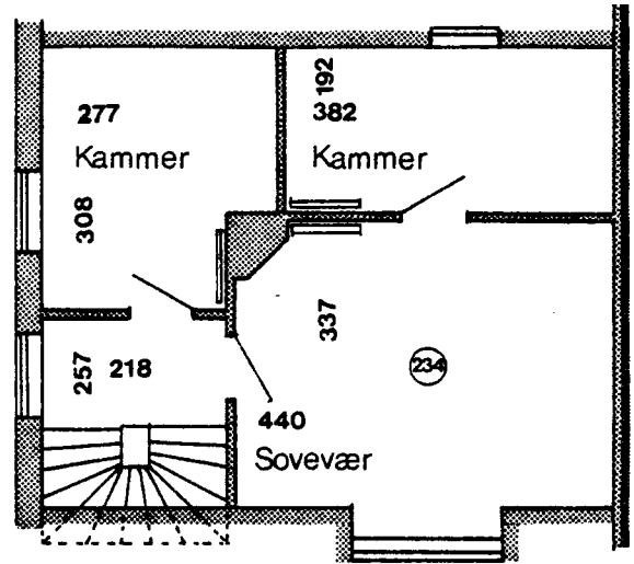
1 Sals plan
