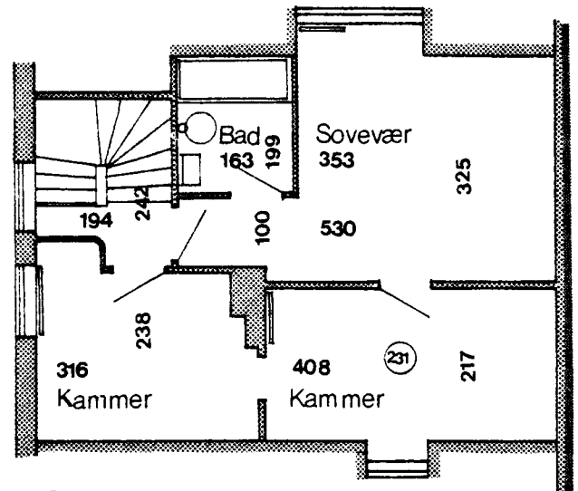
1 Sals plan
