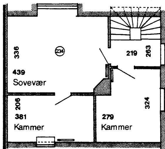
1 Sals plan
