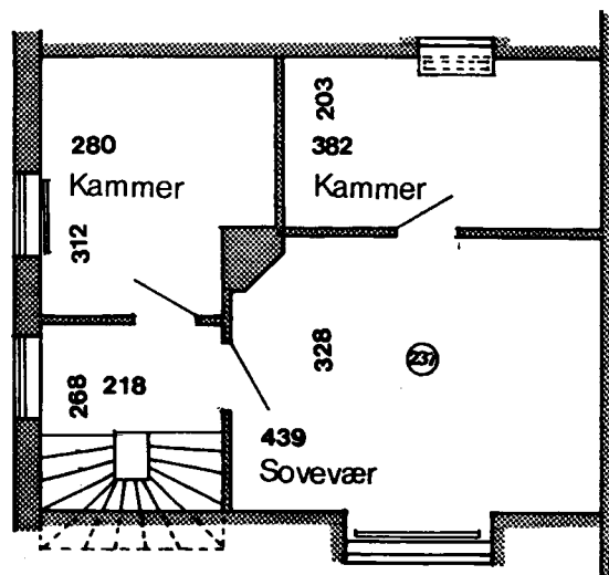
1 Sals plan
